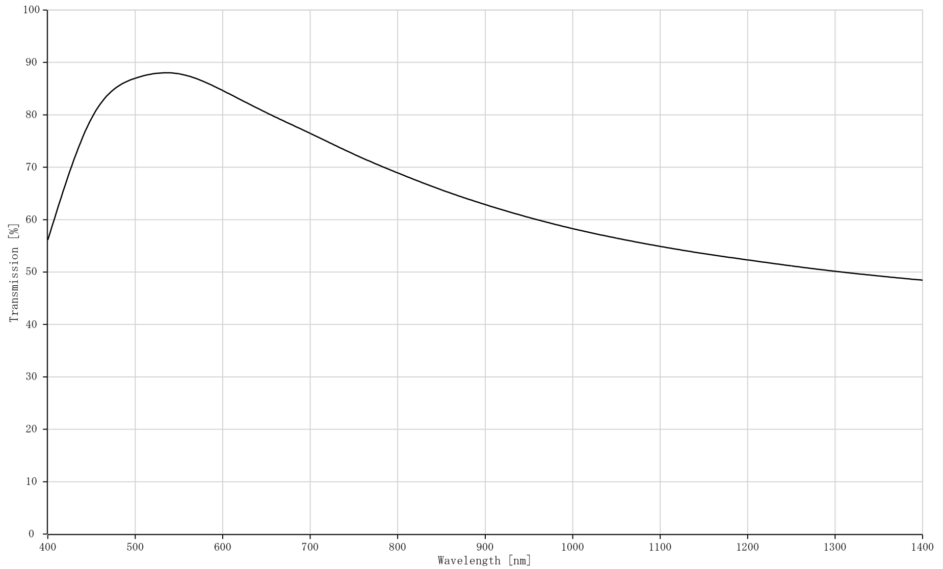
LM16EC-IR Transmission
